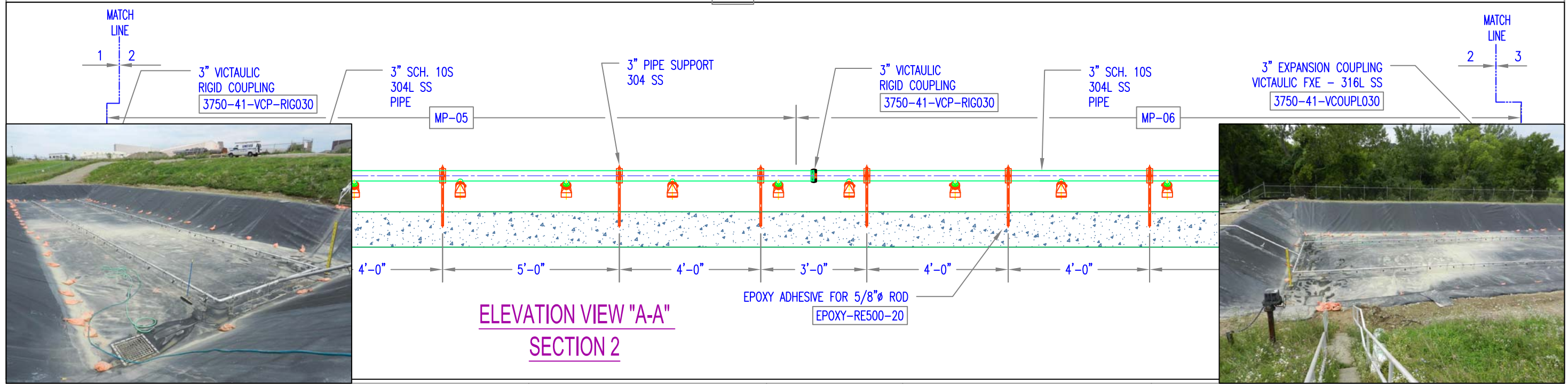
ELEVATION VIEW "A-A"
