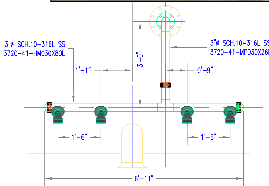
HRMS RECIRC MANIFOLD LEFT SIDE CONFIGURATION HRMS-41-030-LEFT
