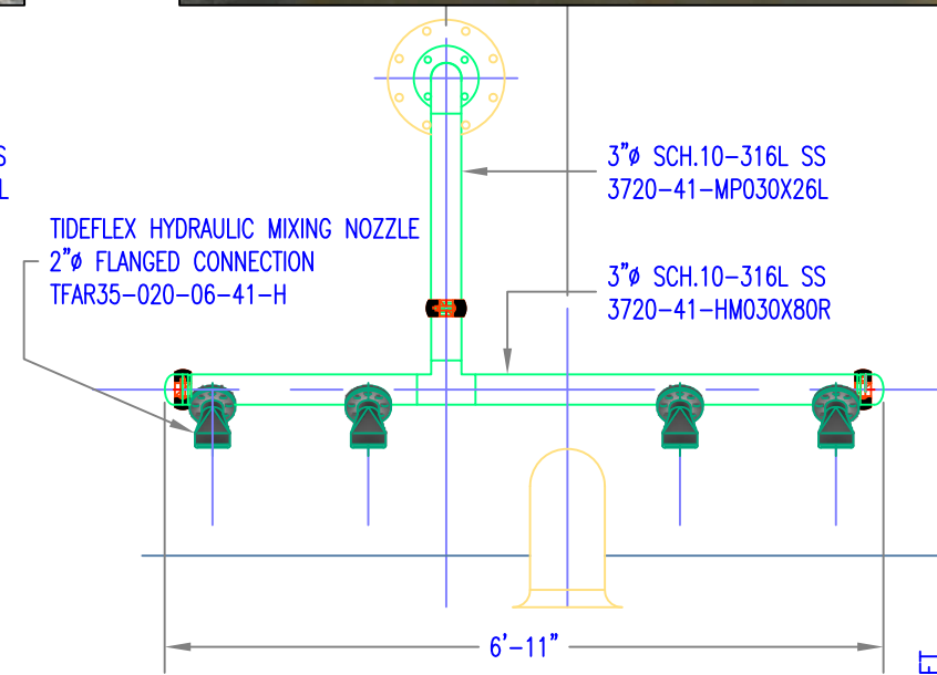
HRMS RECIRC MANIFOLD RIGHT SIDE CONFIGURATION HRMS-41-030-RIGHT
