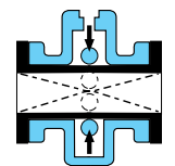
Closing Action
